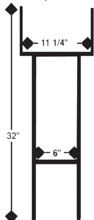
Steel Wide Realtor Wire Stand 32" High
