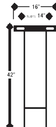
Steel T Post 42" High
